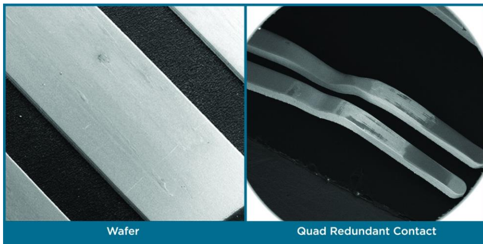
Figure 5. Contacts after 10,000 mating cycle durability testing show acceptable contact surfaces.
