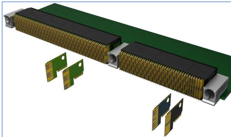
Figure 1. A typical VITA 46 6U VPX configuration uses the MULTIGIG RT 2 connector. The use of wafers in the MULTIGIG RT 2 daughtercard connector helps create a light weight, versatile, pinless connector design.
