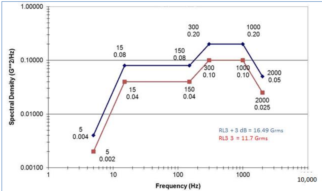
Figure 2. Testing performed by the VITA 72 working group subjected connectors to much more stressful testing with the RL3 + 3 dB level random vibration.
