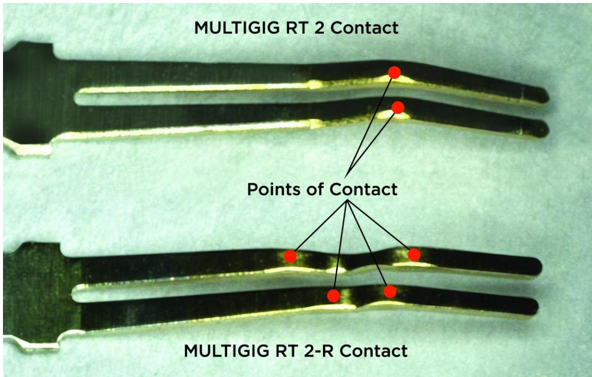
Figure 3. Original and quad redundant MULTIGIG RT 2 contacts
