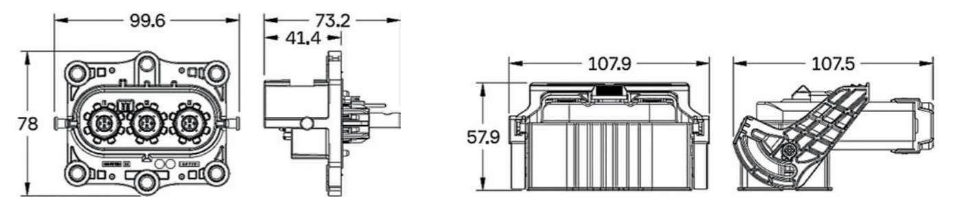
Header Connector
