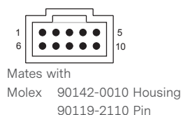
Figure 2. Connector J1
