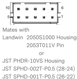
Figure 3. Connector J2
