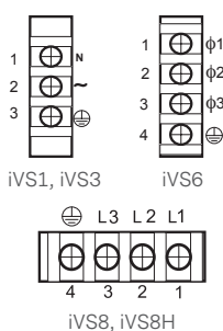
Figure 3. Connector J2
