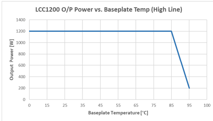
Figure 14. Output Power Vs Baseplate Temperature (High Line: 180 Vac to 264 Vac)
