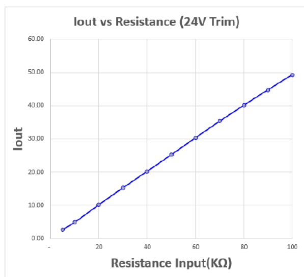
Figure 17. Typical Resistance Dimming using LED load at around 25°C
