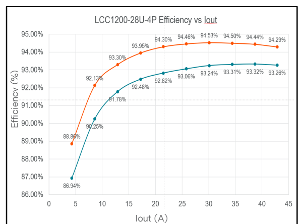
Figure 24: LCC1200-28U-4P Efficiency Curve @ 25°C Loading: I o,max = 10% I o,max increment to 1200W@180/230Vac
