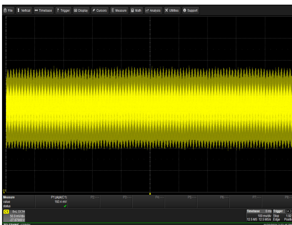
Figure 11: LCC1200-28U-9P Ripple and Noise Measurement Vin = 230Vac Load: Io = 42.9A (12V), I SB = 1.5A (5V) Ch 1: V O
