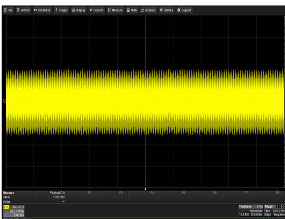
Figure 23: LCC1200-28U-4P Ripple and Noise Measurement Vin = 230Vac Load: Io = 42.9A (28V), I SB = 1.5A (5V) Ch 1: V O
