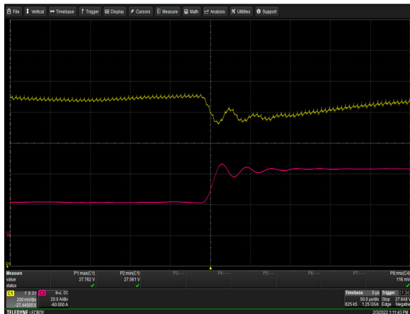
Figure 21: LCC1200-28U-4P Transient Response - Vo Deviation 50% to 100% load change 1A/uS slew rate Vin = 230Vac Ch 1: V O Ch 2: I O
