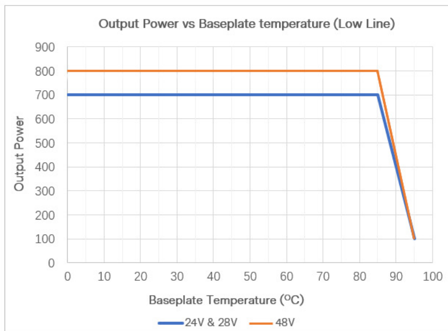
Figure 13. Output Power Vs Baseplate Temperature (low line: 90 Vac to 179 Vac)
