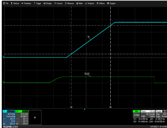
Figure 7: LCC1200-28U-9P Output Startup Characteristic Vin = 264Vac Load: Io = 42.9A (12V), I SB = 1.5A (5V) Ch 3: V O Ch 4: G_DCOK_C
