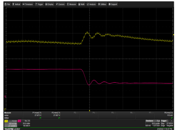
Figure 22: LCC1200-28U-4P Transient Response - Vo Deviation 100% to 50% load change 1A/uS slew rate Vin = 230Vac Ch 1: V O Ch 2: I O
