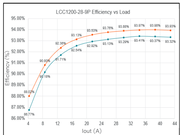
Figure 12: LCC1200-28U-9P Efficiency Curve @ 25°C Loading: I o,main = 10% I o,max increment to 1200W@180/230vac
