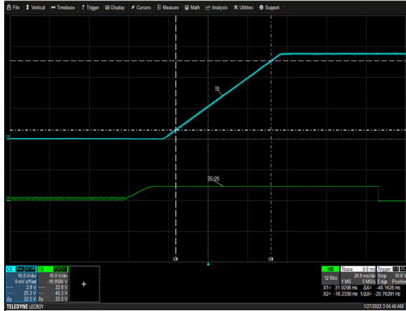
Figure 19: LCC1200-28U-4P Output Startup Characteristic Vin = 264Vac Load: Io = 42.9A (12V), I SB = 1.5A (5V) Ch 3: V O Ch 4: G_DCOK_C
