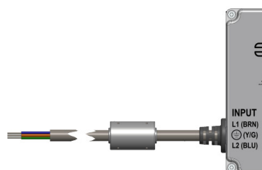
“-4P” Input
