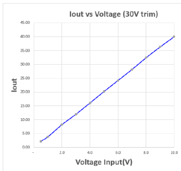
Figure 16. Typical Voltage Dimming using LED load at around 25°C
