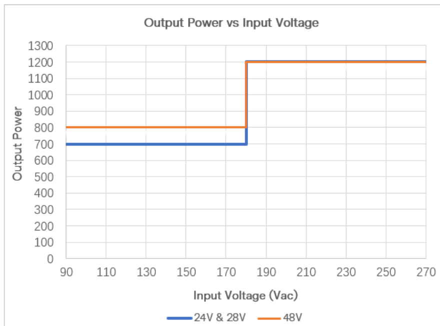
Figure 15. Output Power Vs Input Voltage
