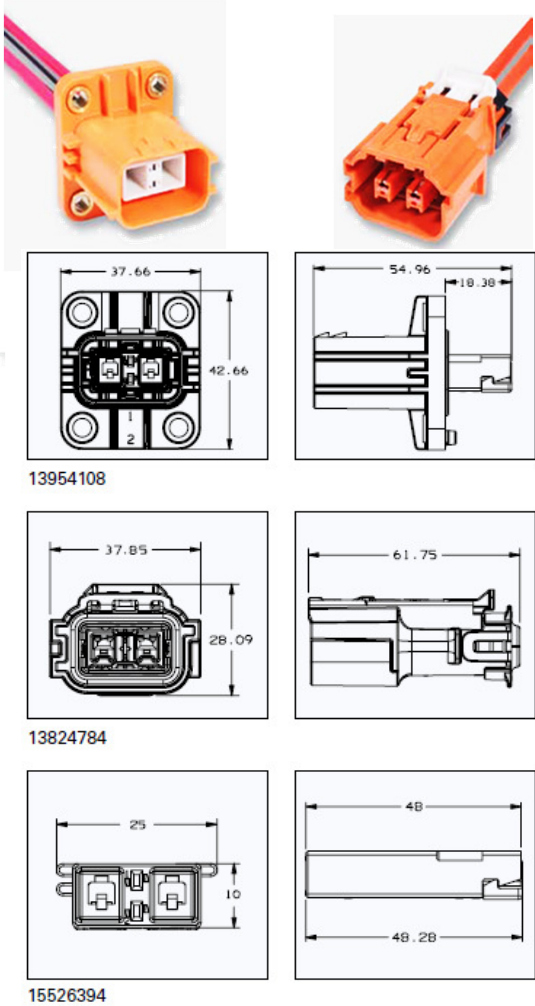
Shield-Pack™ HV280 2 Piece Header with Pluggable Inner Connector
