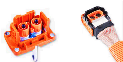
RCS890 High Voltage 2 Way Right Angle Connection System with HVIL
