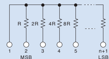
K circuit
