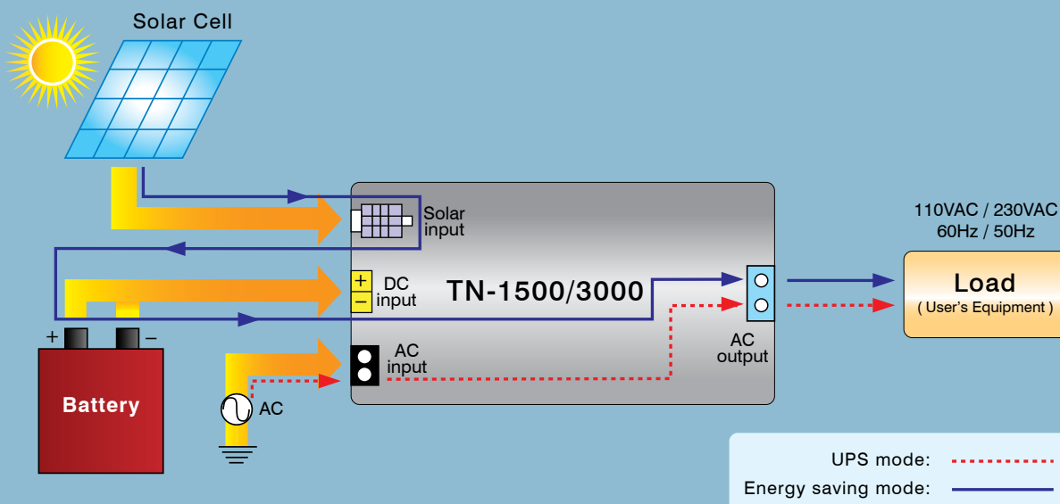
UPS and Energy Saving Block Diagram
