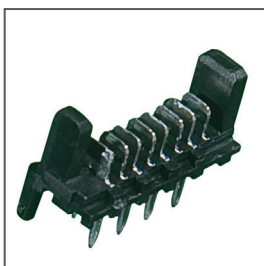
Low profile, vertical, through-hole header Series 90325
