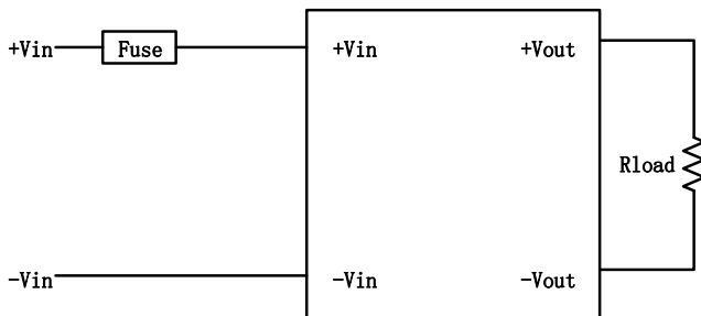
Figure 2. Input Fusing
