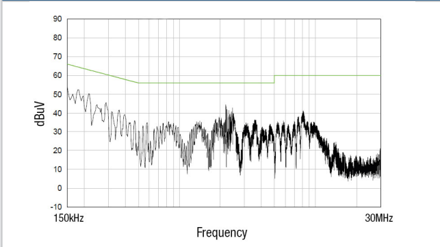
BAC1S12SC (230V) - Live
