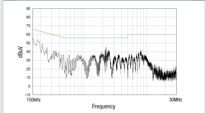
BAC1S12SC (230V) - Neutral
