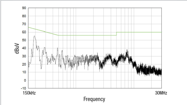
BAC1S12SC (230V) - Live
