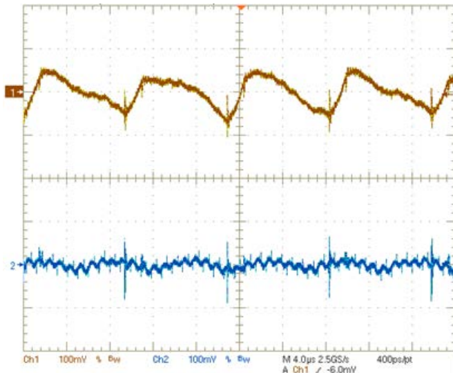
Output Ripple and Noise (Vin = 75V, Iout main = 8A, Iout aux = 1A, Cload = 0.1uF, Scope Bandwidth = 20MHz) Trace 1 = Vout main, Trace 2 = Vout aux
