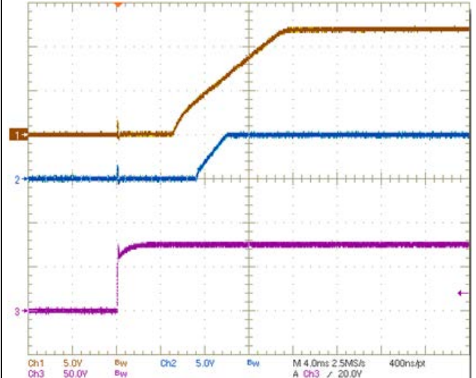
Turn On Delay (Vin = 75V, Iout main = 8A, Iout aux = 1A, Cload = 0.1uF) Trace1 = Vout main, Trace 2 = Vout aux, Trace 3 = Vin
