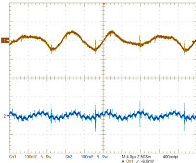
Output Ripple and Noise (Vin = 36V, Iout main = 8A, Iout aux = 1A, Cload = 0.1uF, Scope Bandwidth = 20MHz) Trace 1 = Vout main, Trace 2 = Vout aux
