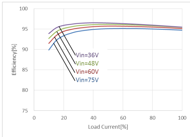
Efficiency vs, Line Voltage and Load Current @Ta = +25°C (100% : Vout12=10A,Vout5=1A)
