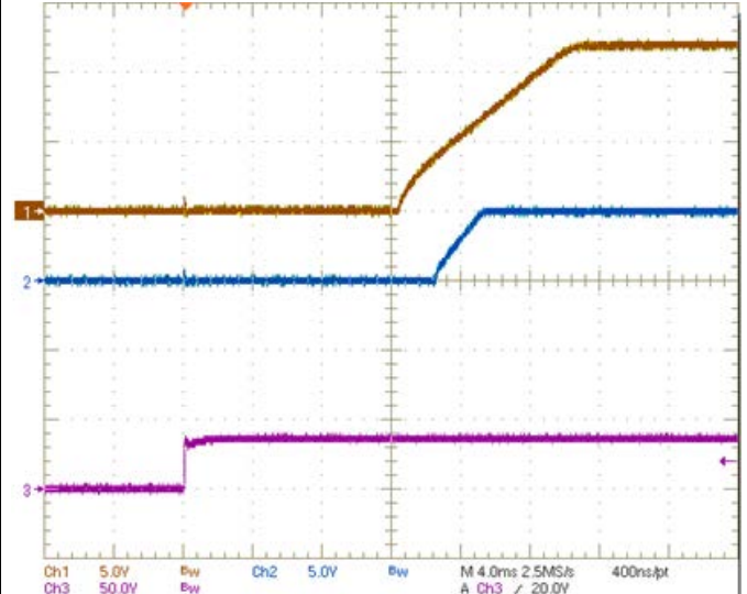
Turn On Delay (Vin = 36V, Iout main = 8A, Iout aux = 1A, Cload = 0.1uF) Trace1 = Vout main, Trace 2 = Vout aux, Trace 3 = Vin
