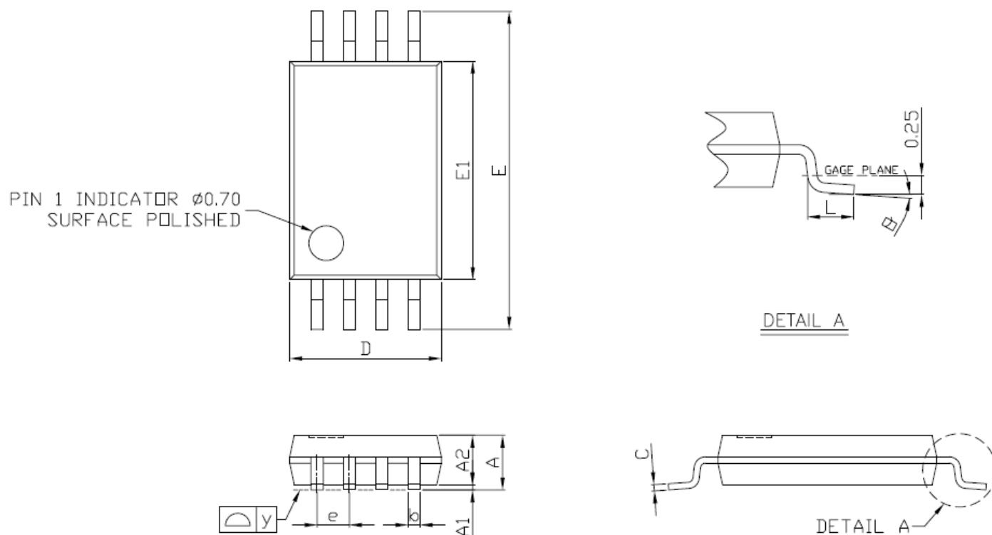
Figure 13. TSSOP-8 Package Drawing
