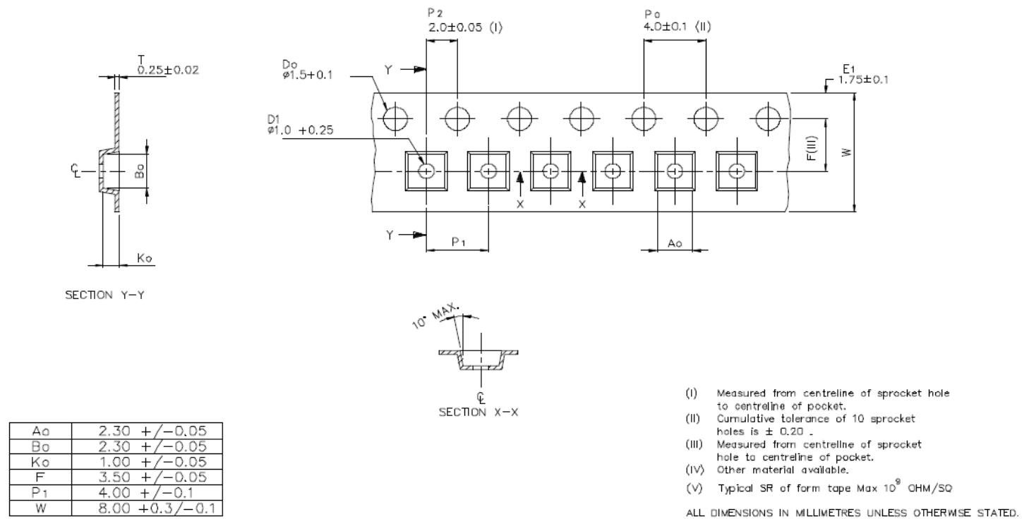
Figure 16. DFN-8 Tape and Pocket Drawings
