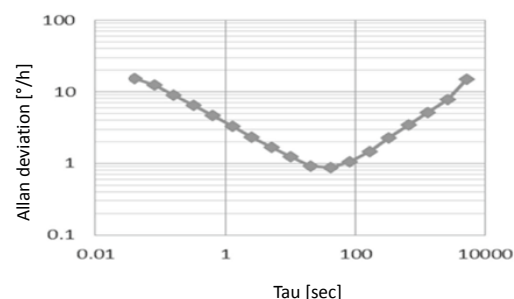
Z-Gyro (SCHA634-D01) Allan Deviation in °/h
