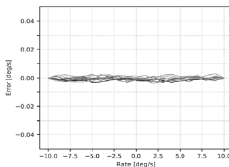
Z-Gyro (SCHA634-D01) Linearity error in deg/s
