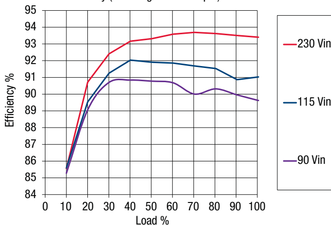
MVAC400-24 Efficiency (including 5V Aux Output)
