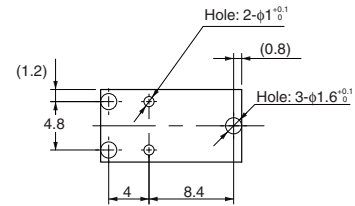
PWB processing dimension (BOTTOM VIEW)
