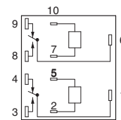
Terminal arrangement / Internal connections (BOTTOM VIEW)
