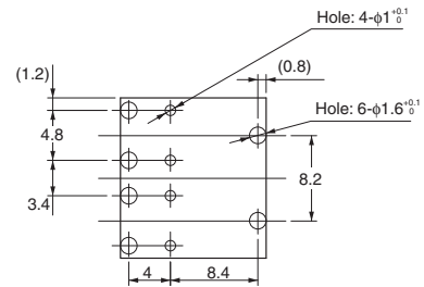
PWB processing dimension (BOTTOM VIEW)
