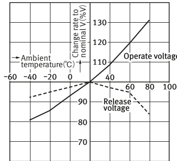
4-2. Ambient temperature characteristics (1 Form A 1 Form B, 2 Form A: Average)
