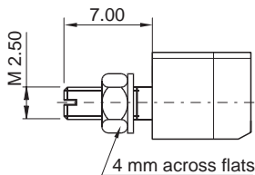
Mass and power contact (molding B)
