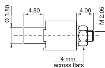
Rotating jackscrew
