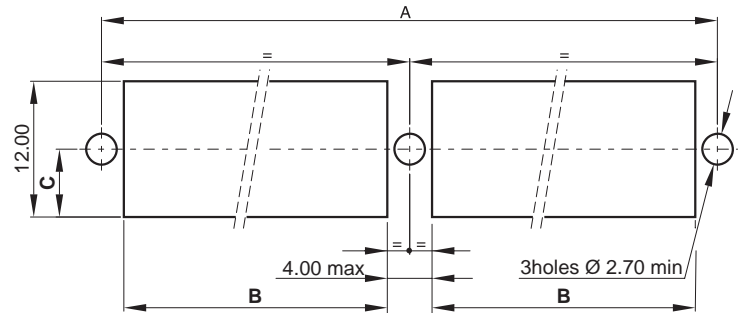
108 to 160 contacts
