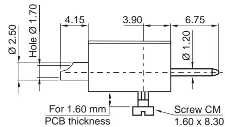
Mass and power contact (molding A)
