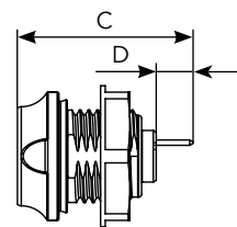
Female Insulator
