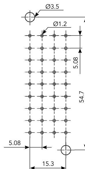
36 contacts
