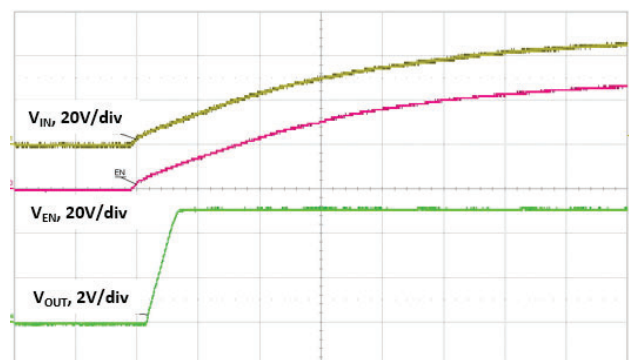
Fig. 30 - Start-up with VIN, Time = 5 ms/div
