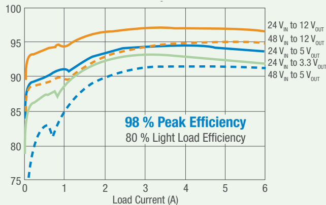
SiC462 Efficiency at 300 kHz
