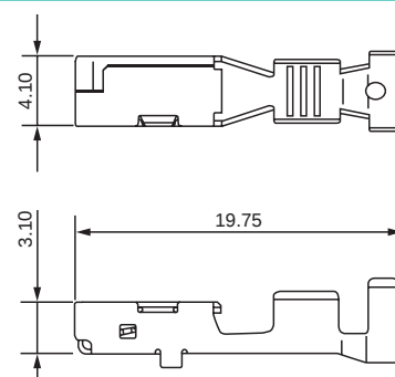
Female Terminal
