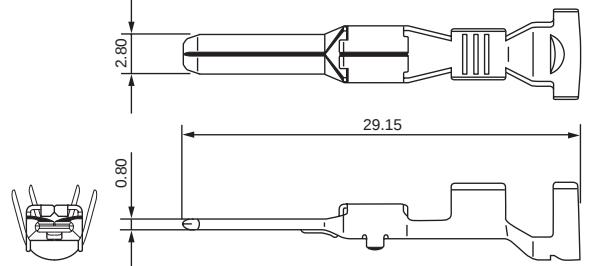
Male Terminal
