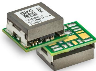
Figure 1 PNA product Size: 13.0 x 12.35 x 6.2 mm (0.512 x 0.486 x 0.244 in)
