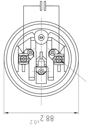
clamp-combi-screw M5x12
