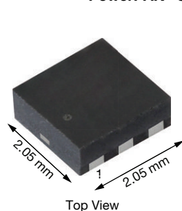
PowerPAK® SC-70W-6L Single
