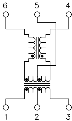
SCHEMATIC
