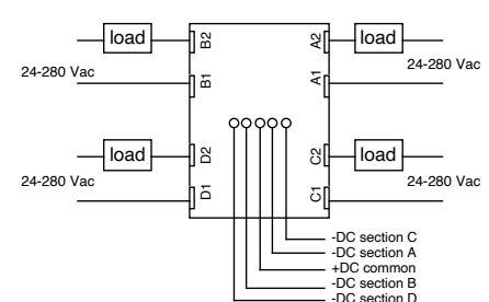
Figure 3: Typical application
