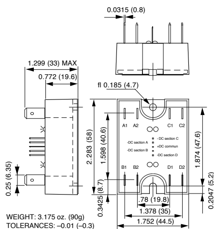
Figure 1: Mechanical specification
