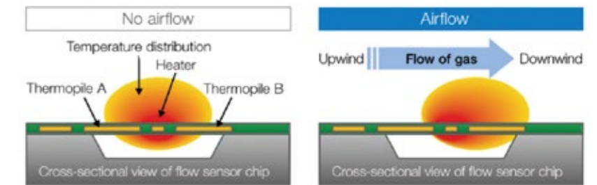
Thermopile technology: the heart of Omron's MEMS flow sensor
