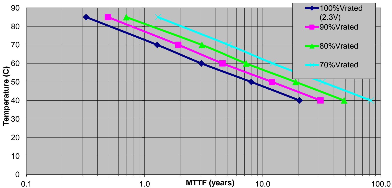
Expected Lifetime at Various Voltages SCC series, 2.3V Rated
